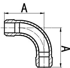
Bend 90°, male
