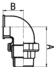
Union Elbow M/F
