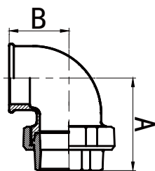
Union Elbow F/F
